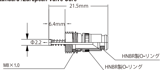
Standard /European Valve Core
