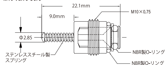
M10 Valve Core
