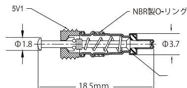
Standard Valve Core
