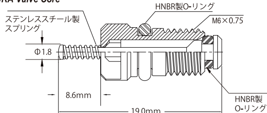
JRA Valve Core
