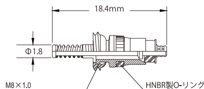
Standard /European Valve Core
