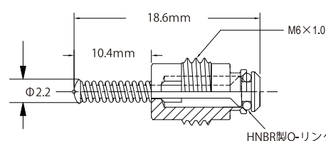
Standard Valve Core
